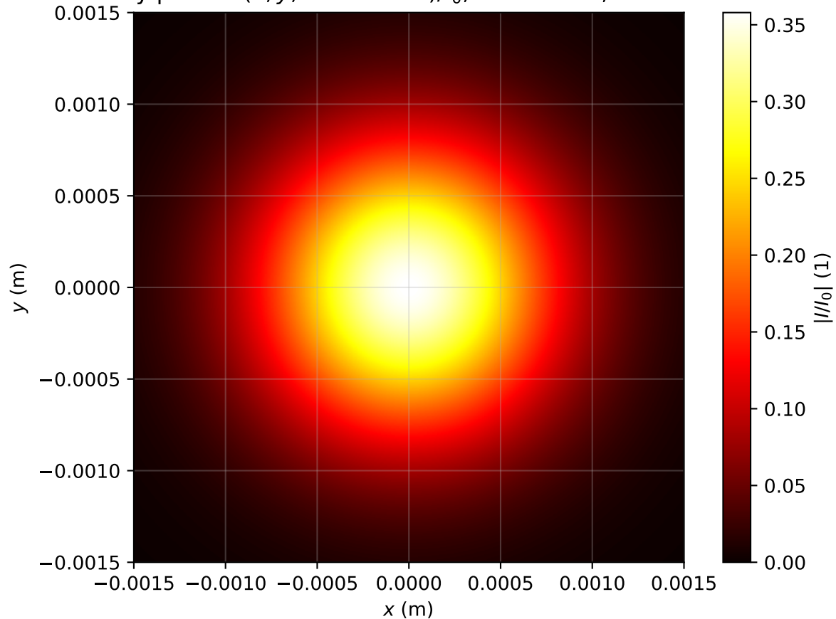
Intensity profile I(x, y, z = 3.105m)/I_0 , P_{in}=0.2P_{cr} , artificial time
